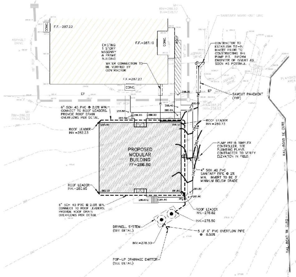
Burnet Hill Elementary School – Site Plan
